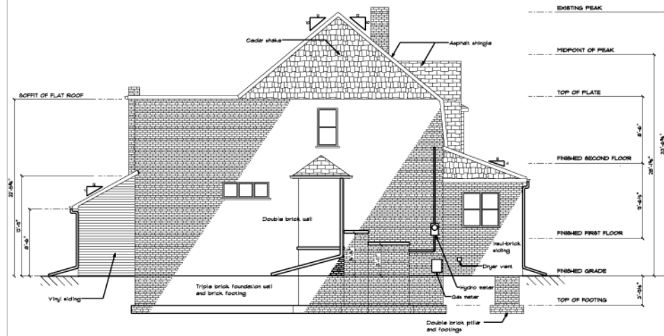
NORTH ELEVATION
